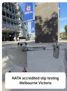
Dry Floor Friction Testing AS 4586 and AS 4663
